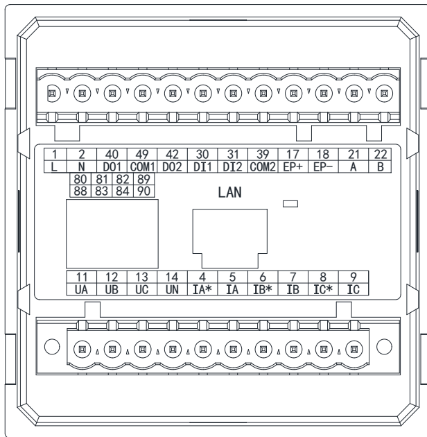
Figure 11 APM510 extended CE wiring diagram
