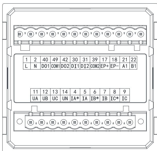
Figure 7 APM510 basic wiring diagram
