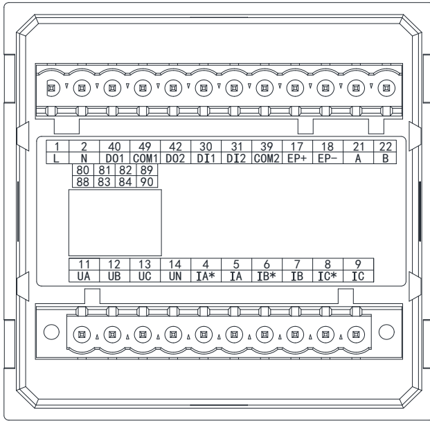
Figure 9 APM510 extended Ethernet/temperature measurement/leakage wiring diagram
