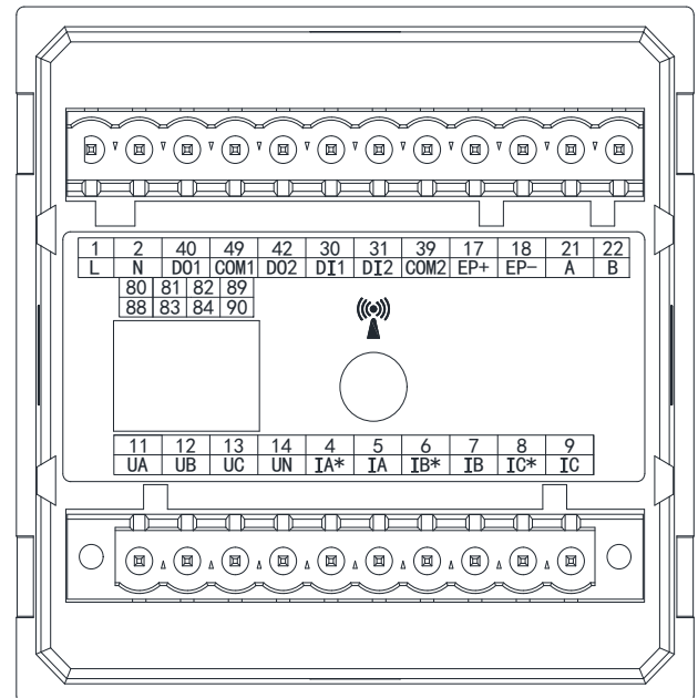
Figure 12 APM510 extended WF/LoRa wiring diagram
