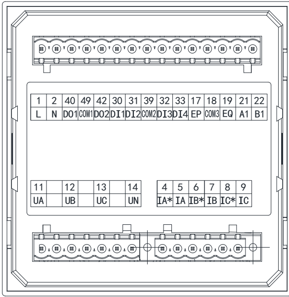
Figure 13 APM520 basic wiring diagram
