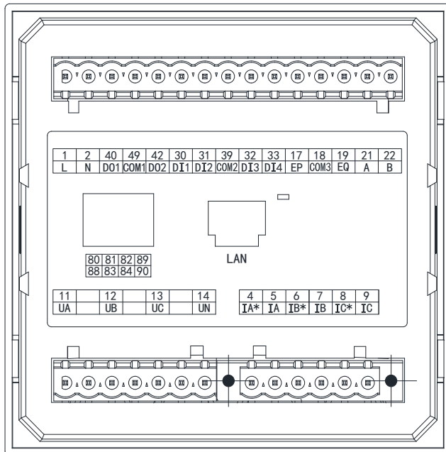
Figure 17 APM520 Extended CE Wiring Diagram
