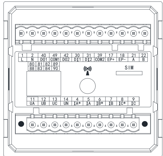
Figure 10 APM510 extended 4G wiring diagram
