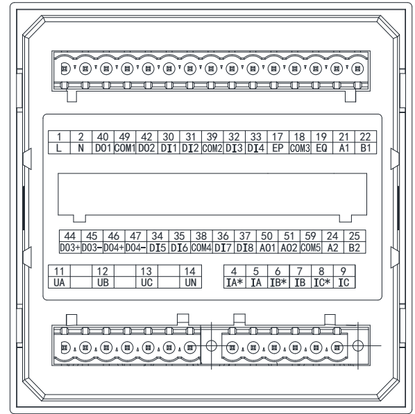
Figure 14 APM520 extended K/2M/2C wiring diagram
