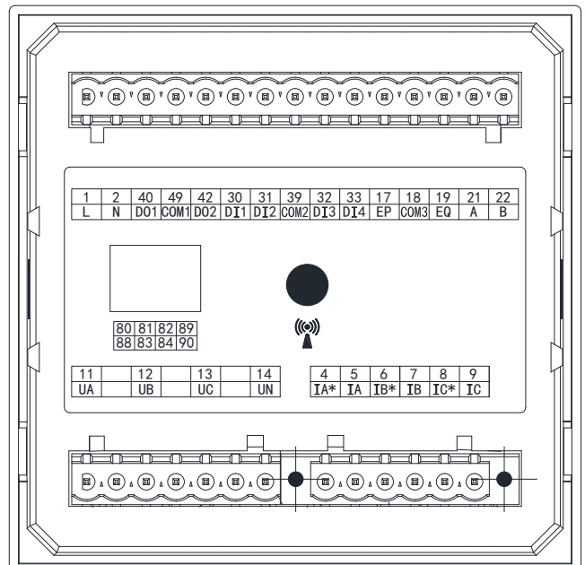
Figure 18 APM520 Extended WF/LoRa Wiring Diagram
