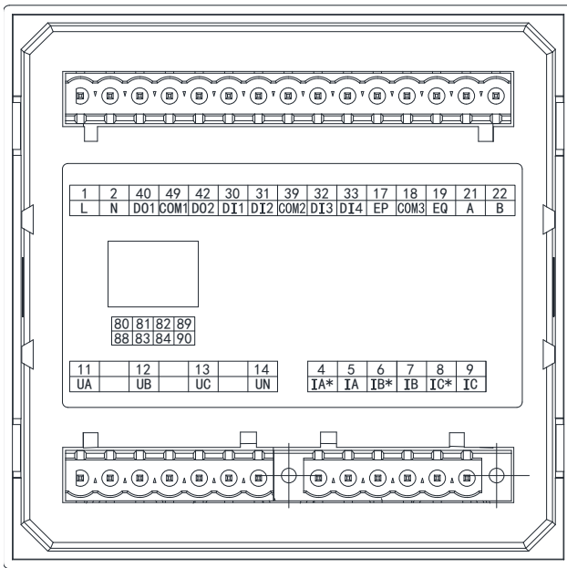
Figure 15 APM520 Extended Ethernet/Temperature Measurement/Leakage Wiring Diagram
