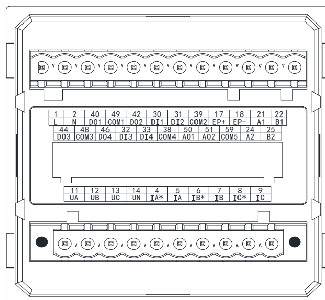
Figure 8 APM510 extended K/2M/2C wiring diagram
