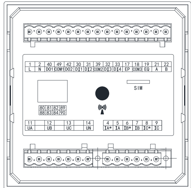
Figure 16 APM520 Extended 4G Wiring Diagram
