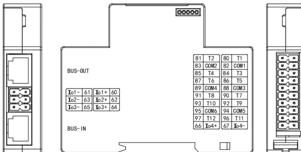
Fig 7 ADW600-TL Wiring Diagram
