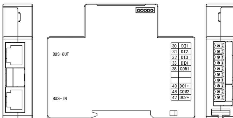
Fig 6 ADW600-K Wiring Diagram
