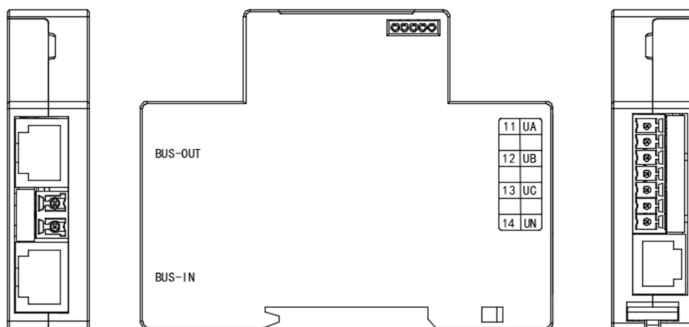
Fig 4 ADW600-U Wiring Diagram
