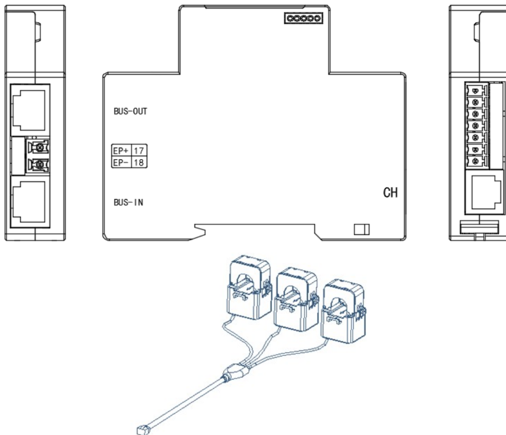
Fig 5 ADW600-I Wiring Diagram
