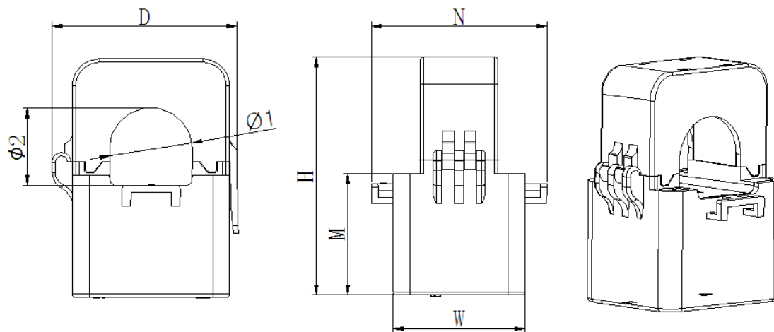
Fig 3 The external dimensions of the accompanying transformer
