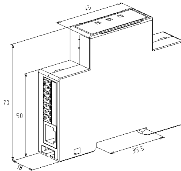
Fig 2 ADW600 dimensional drawing
