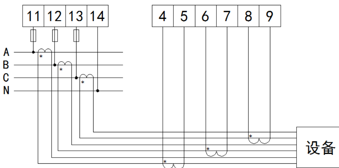
3-phase 4-wire
