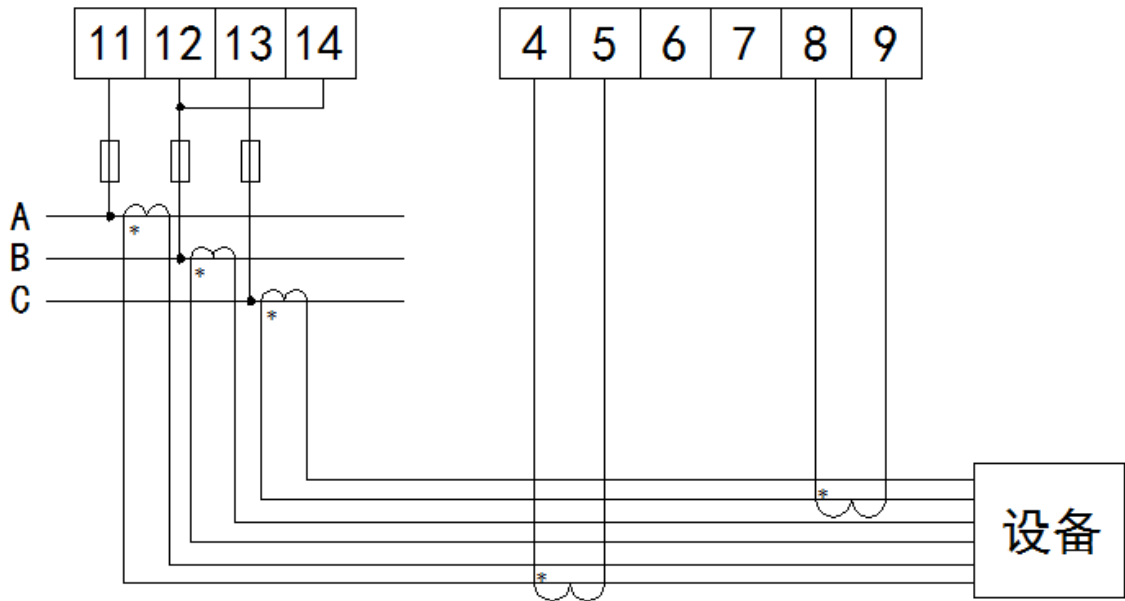
3-phase 3-wire
