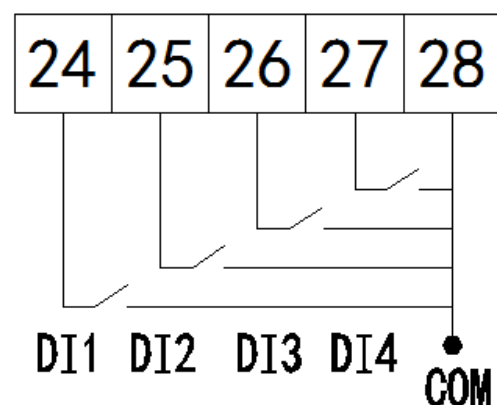
Digital input
