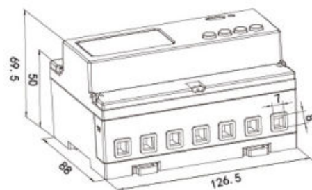
Direct connect
