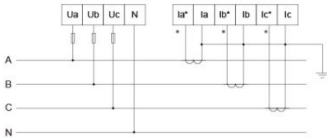
Three phase four lines connect via CT
