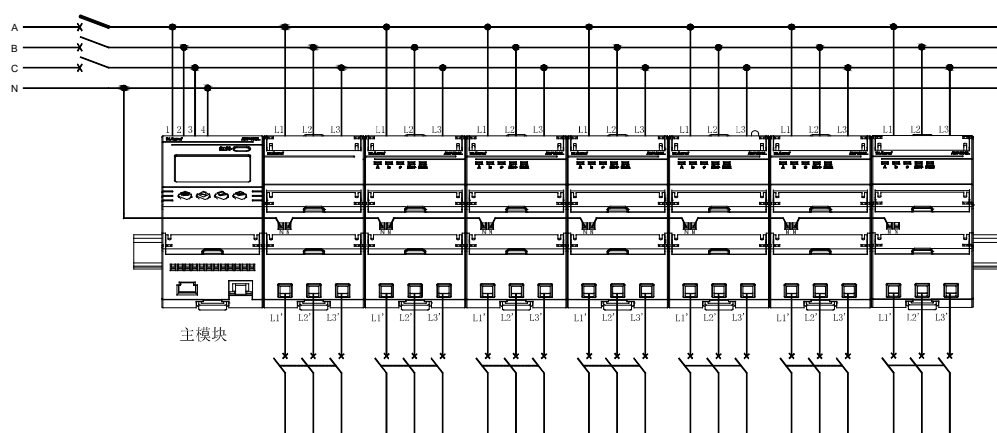
36-channel single item direct access diagram
