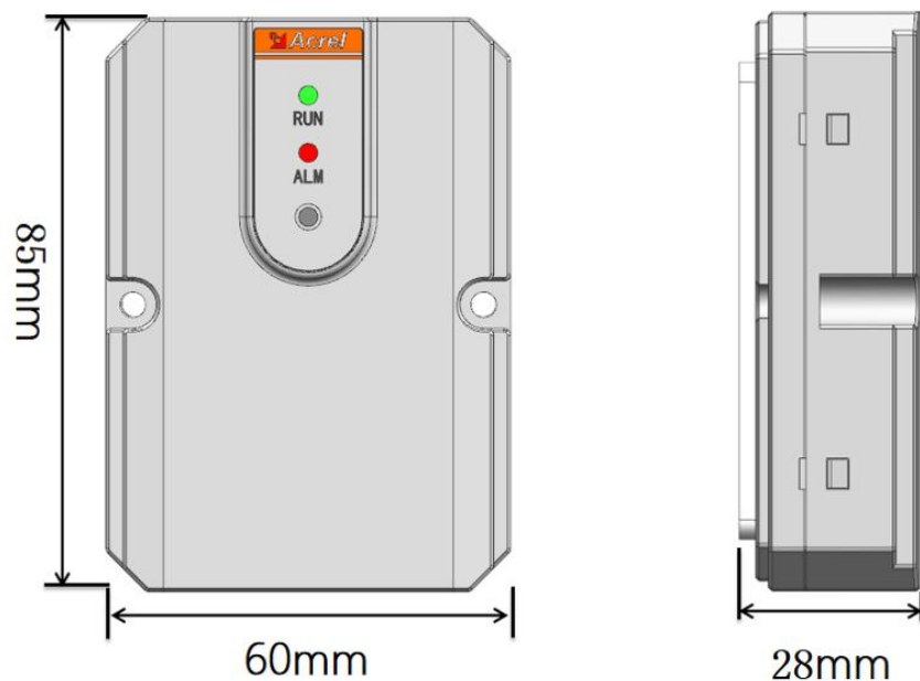
Fig.1 Dimensions of ABAT100 series module
