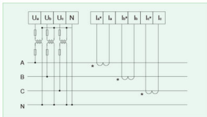
Three-phase four-wire
