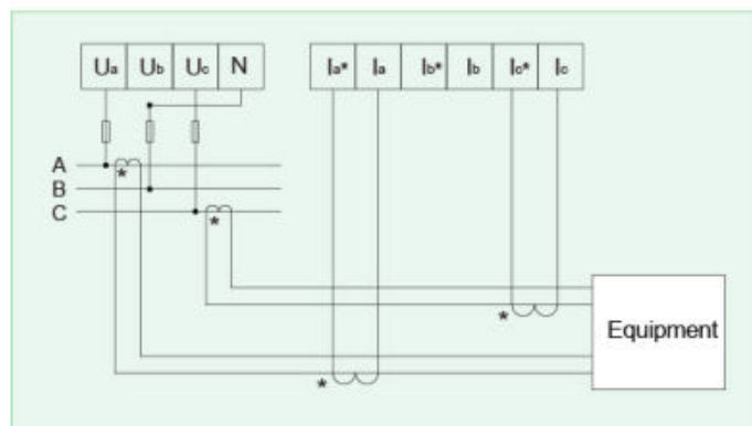
Three-phase four-wire
