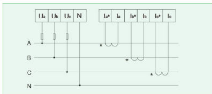
Three-phase four-wire
