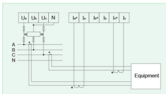
Three-phase three-wire
