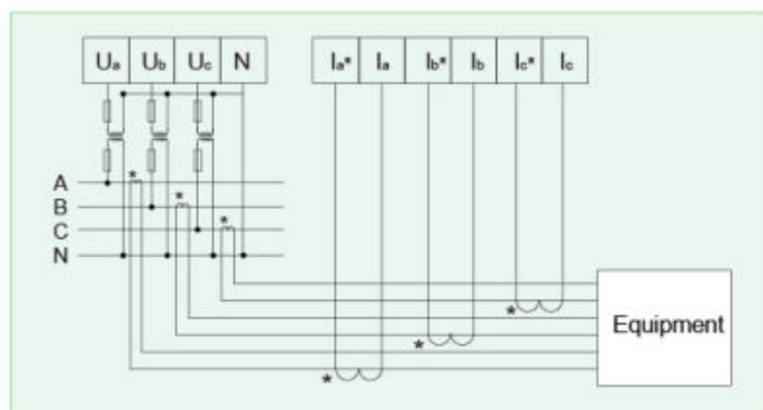
Three-phase three-wire
