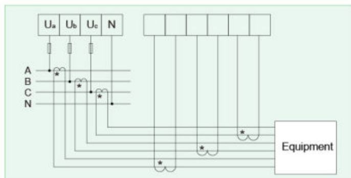
Three-phase four-wire
